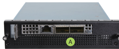
A 2x 100GbE QSFP56
