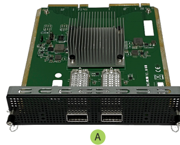
A 2x 100 GbE QSFP28
